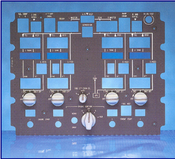
C-17 Globemaster NVIS compatible panel.
