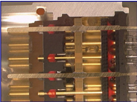
Connector cross-section
